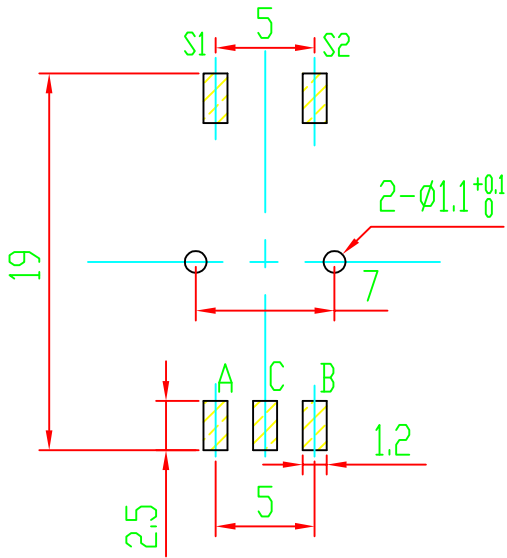
P.C.B MOUNTING DETAIL
