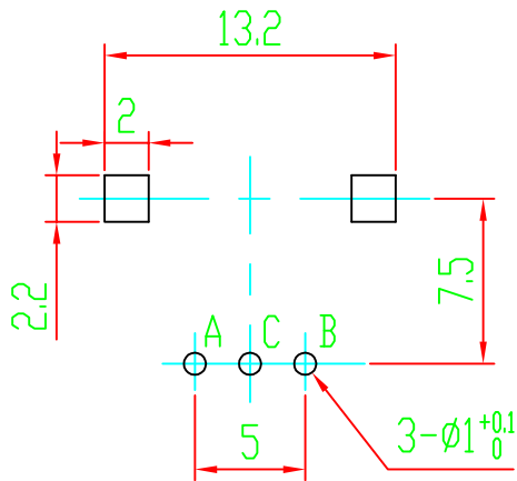
P.C.B MOUNTING DETAIL
